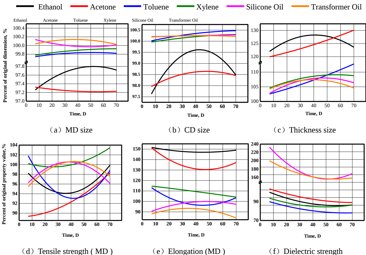
► Figure 6 Chemical stability of Metastar ® YT510-0.08mm Paper
